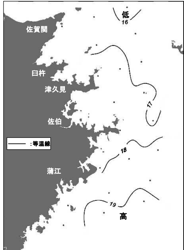
50m層水温
